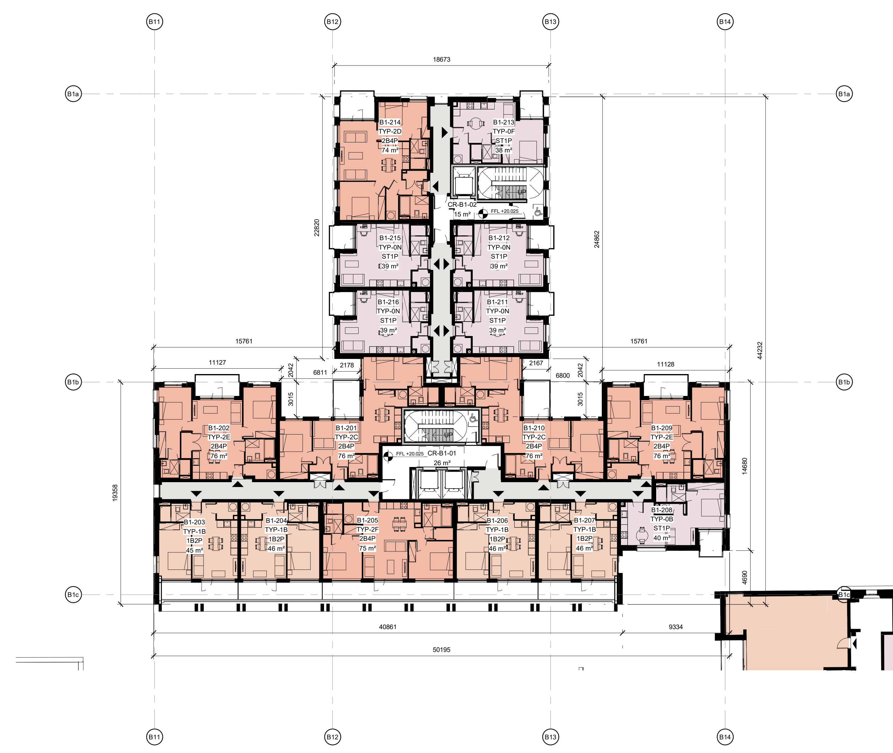
3 BLOCK B1-LEVEL 02 1 : 200
