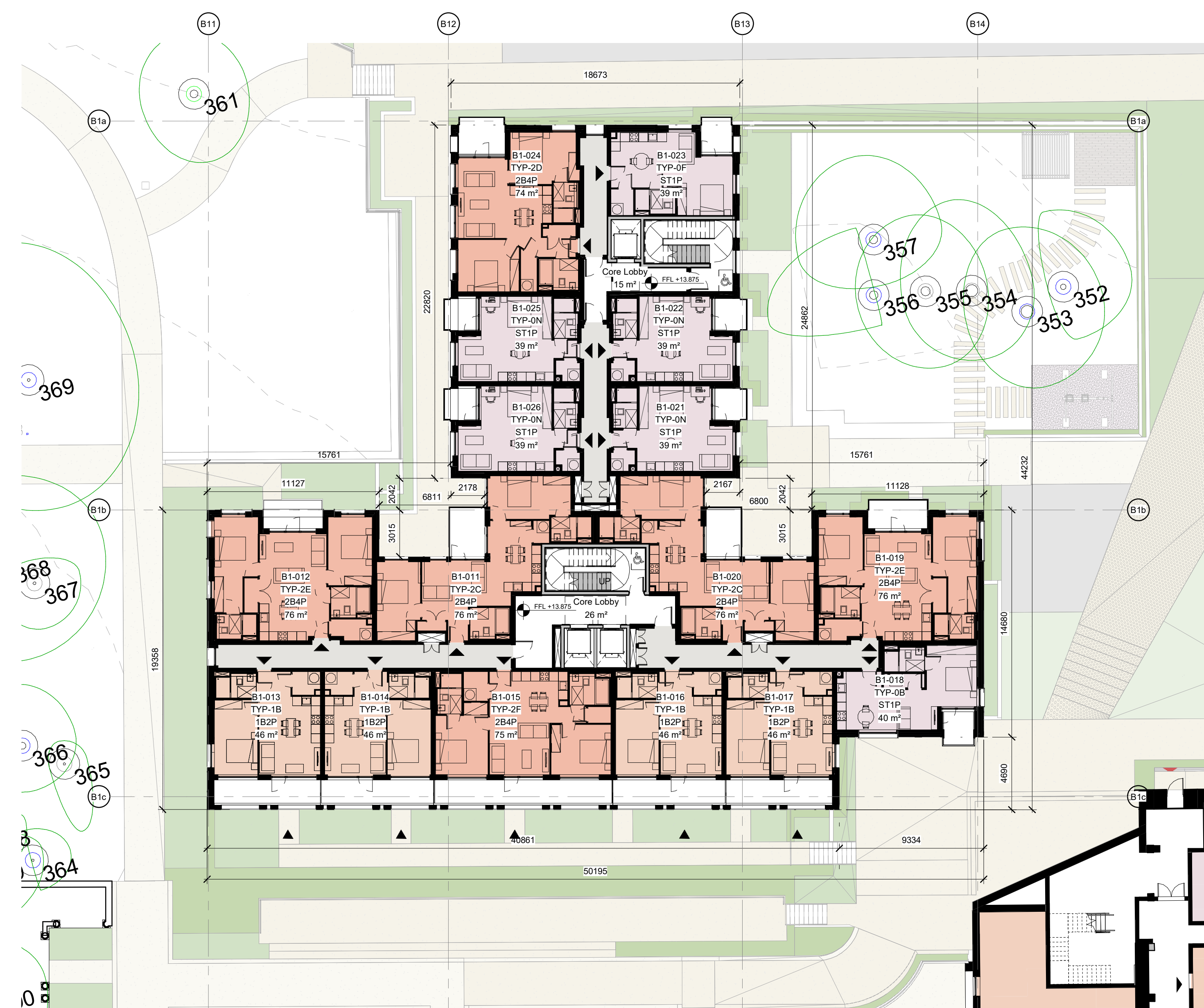
2 BLOCK B1-LEVEL 00 1 : 200
